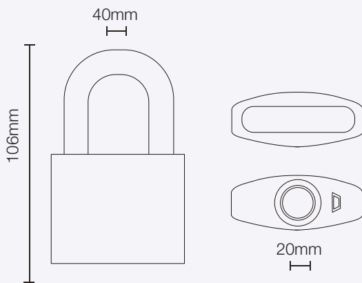
AEG-SPL-P207 STAINLESS STEEL SHACKLE Unit Price RM360 (30 pc/carton)
